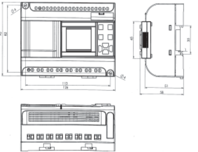
Fig 2.3 AF-20 FAB Series installation dimensions (Unit: mm)
