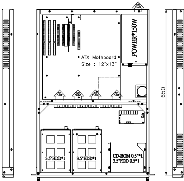
Left View
