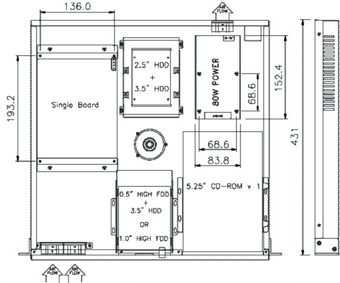
Top View
