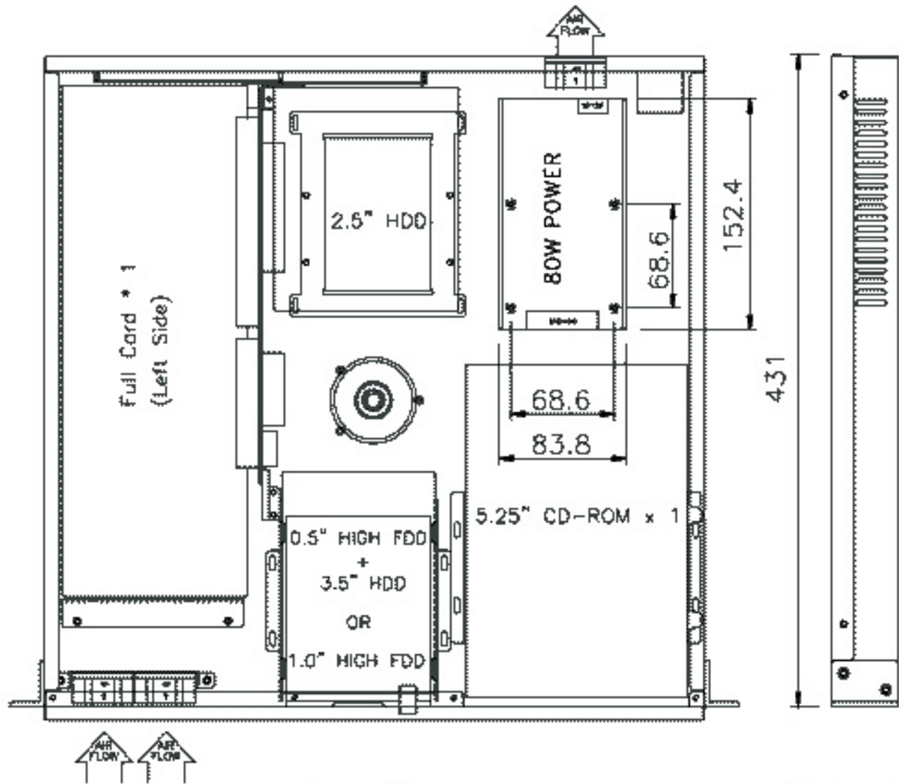
Top View
