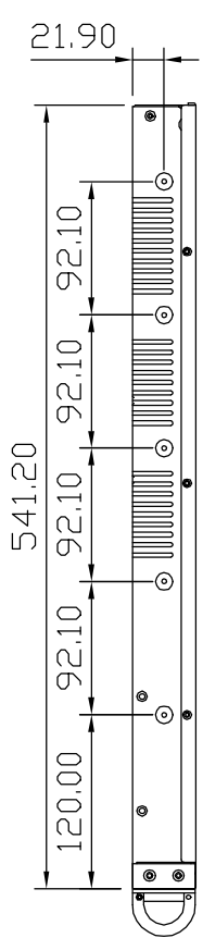
Left View
