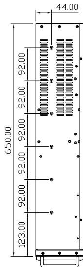
Left View
