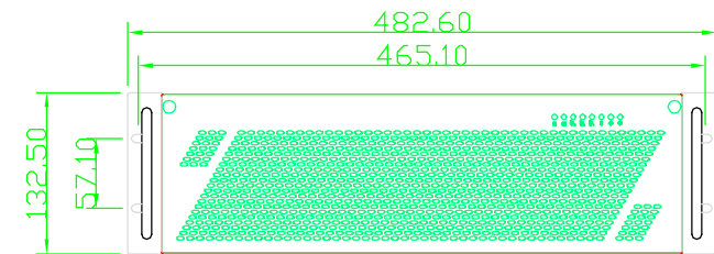
Front out-side View
