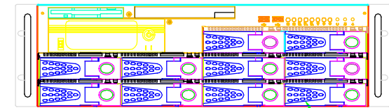
Front in-side View 3.5HDD x 10
