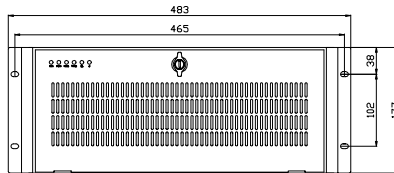
Front out-side view
