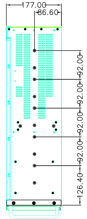
Right-side View
