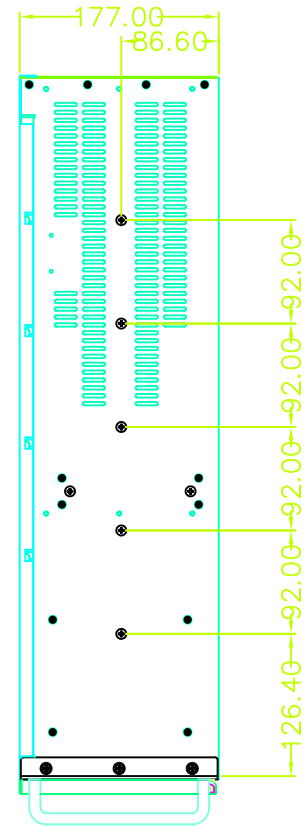
Right-side View
