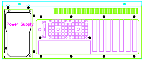
Rear view
