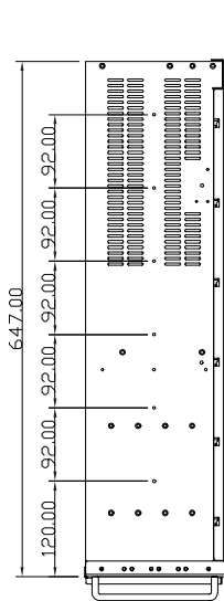
Left View
